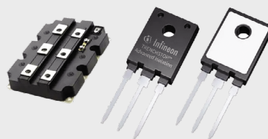
IGBT 封裝
